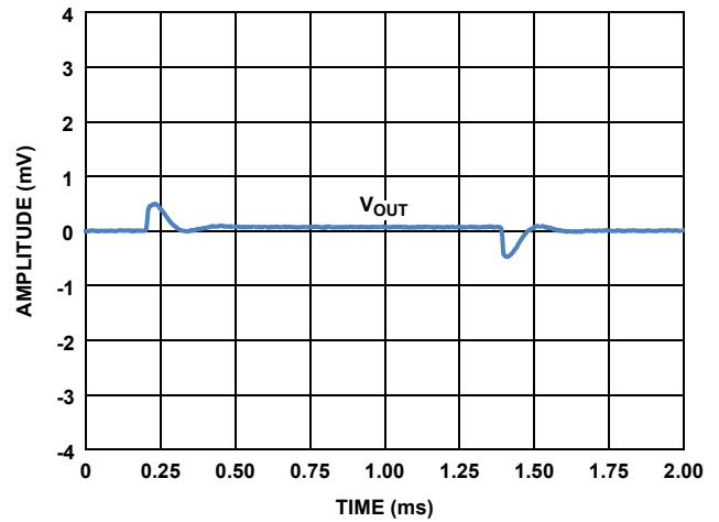
FIGURE 16. LINE TRANSIENT ( \Delta V_{IN} = 500mV )
