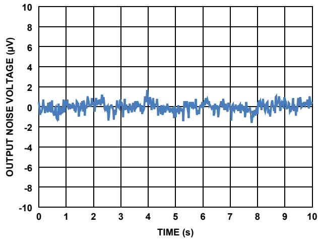
FIGURE 21. V_{OUT} vs NOISE, 0.1Hz TO 10Hz
