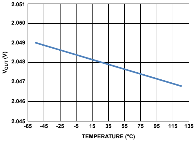
FIGURE 22. SIMULATED (WORSE CASE) V_{OUT} vs TEMPERATURE
