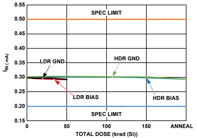
FIGURE 4. SUPPLY CURRENT SHIFT
