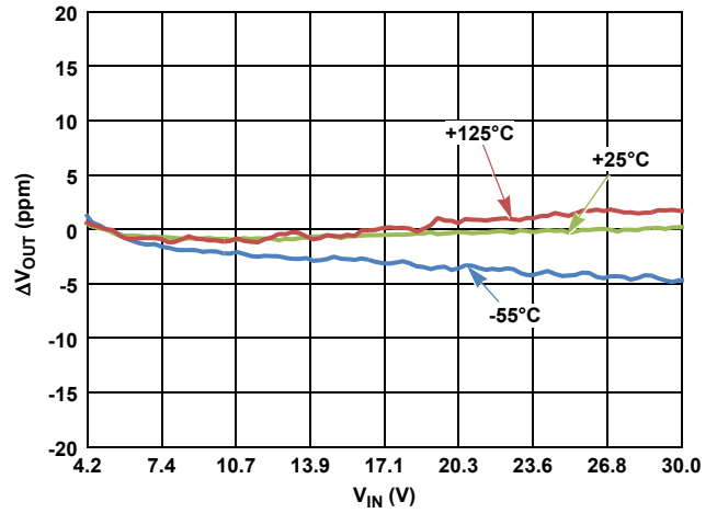
FIGURE 10. LINE REGULATION vs \Delta V_{OUT} (PPM) OVER-TEMPERATURE
