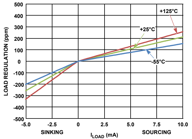
FIGURE 12. LOAD REGULATION vs V_{OUT} (PPM) OVER-TEMPERATURE
