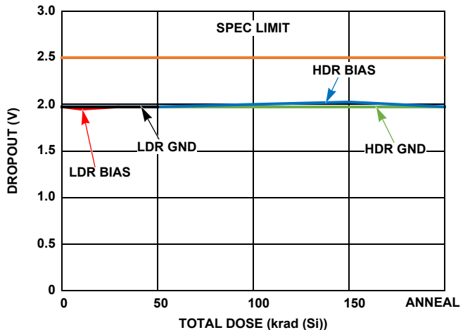
FIGURE 8. DROPOUT SHIFT
