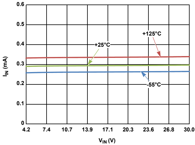
FIGURE 15. I_{IN} vs V_{IN} OVER-TEMPERATURE
