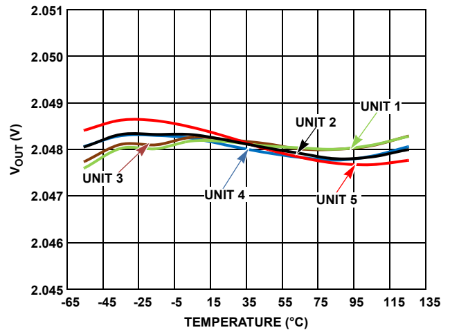
FIGURE 14. V_{OUT} vs TEMPERATURE
