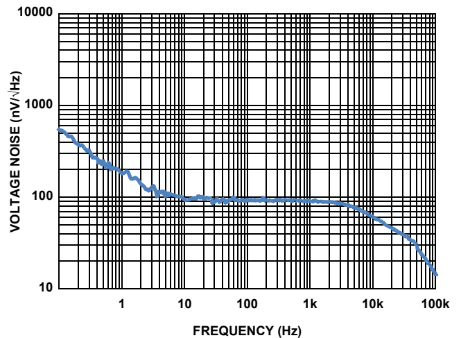
FIGURE 20. NOISE VOLTAGE DENSITY vs FREQUENCY
