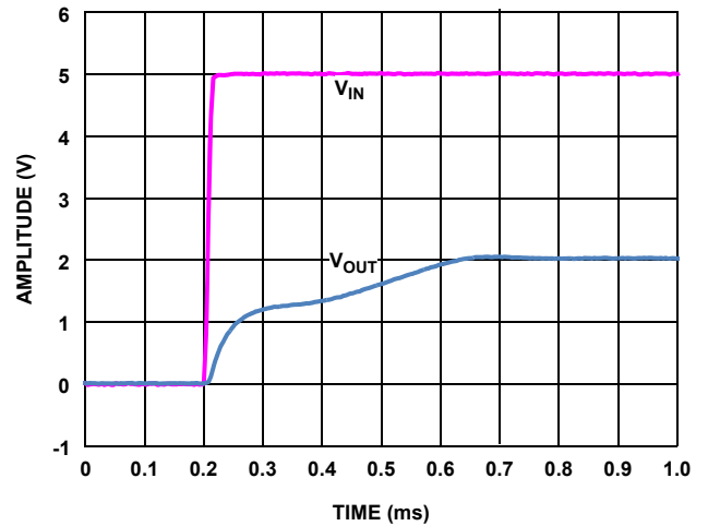
FIGURE 18. TURN-ON TIME
