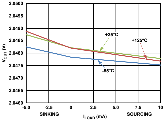
FIGURE 11. LOAD REGULATION vs V_{OUT} (V) OVER-TEMPERATURE
