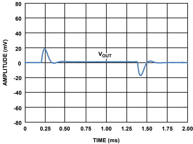
FIGURE 17. LOAD TRANSIENT ( \Delta I_L = 1mA )
